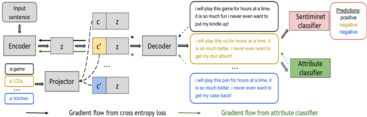
Figure 1. provides an overview of our adversarial examples generation technique.
